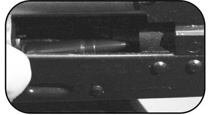
Round being stripped from magazine.
