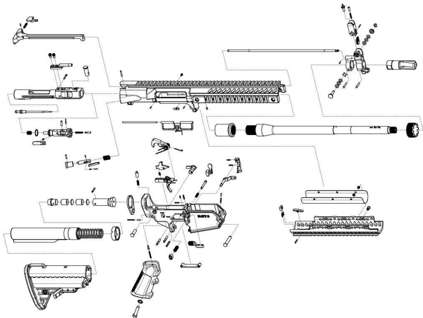
Exploded View
