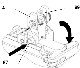
To fold down, push in on button (67) and fold down sight
