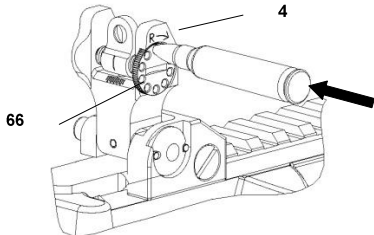
To adjust for windage, use bullet tip or coin to rotate windage adjustment knob
