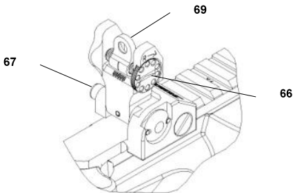
Backup Iron Sight (BUIS) adjustable for windage only
