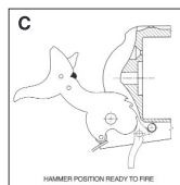
HAMMER POSITION READY TO FIRE
