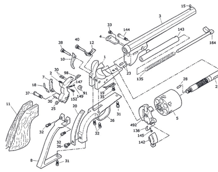
MODEL 1851 RICHARDS-MASON CONVERSION
