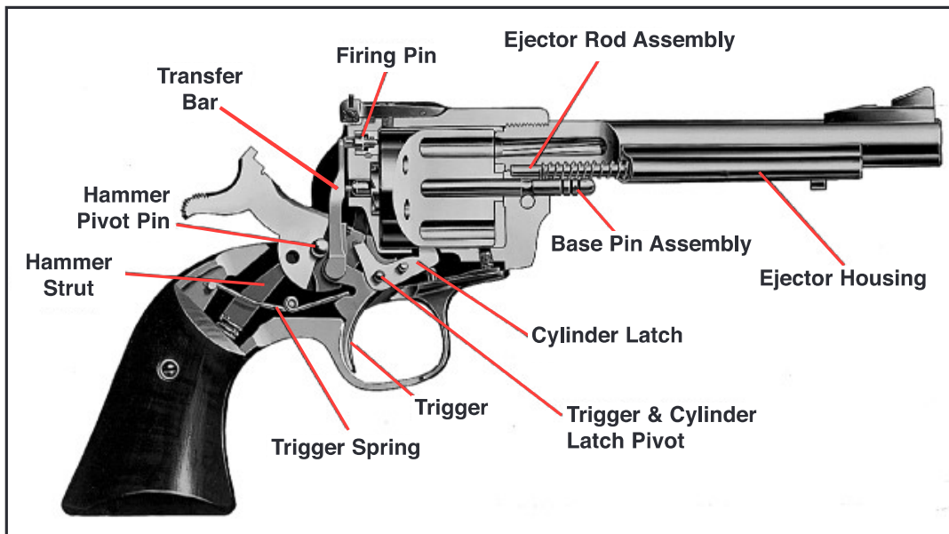
Figure 2. Mechanism shown with trigger pulled and hammer beginning to fall. The transfer bar is in firing position, between the hammer and firing pin.
