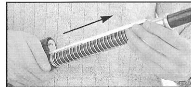
Fig. 17: With the cocking handle removed from the bolt you can grasp the piston, slide the bolt and action bar forward and remove the assembly from the
