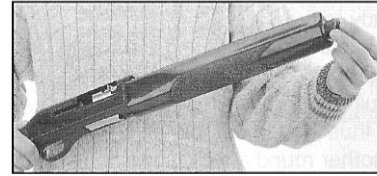
Fig. 15: With the bolt in the forward position, unscrew the forend cap and remove the forend. Remove the barrel by pulling the barrel and barrel extension out of the receiver.
