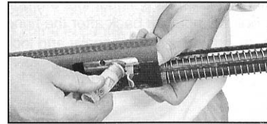
Fig. 16: Use a flathead screwdriver to remove Bolt Cocking Handle. You will see a notch on the backside of the handle.
