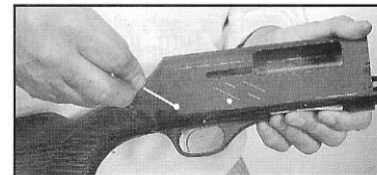
Fig. 18 & Fig. 19: The trigger assembly can be removed
