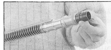
Fig. 14: The gas piston assembly on the magazine tube. These parts must be cleaned and lightly oiled after each use. Inspect the
