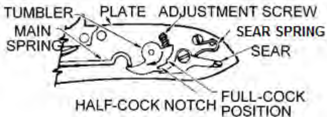
Internal Lock Parts
