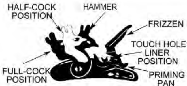
FLINTLOCK: EXTERNAL LOCK PARTS
