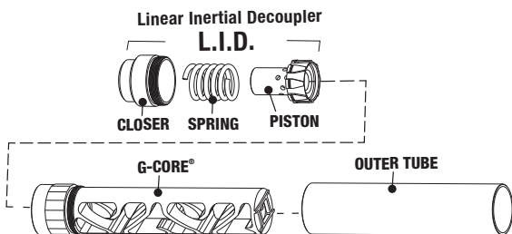
GM™ -45 Assembly Diagram
